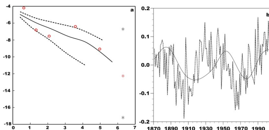
Fig. 3: a) The results of the statistical test on the significance of the Intrinsic Mode Function of the summer MO index. Symbols, lines and axes as in Fig. 1a. b) Evolution in time of the phase inverted 4th IMF of the EMD of the summer (JJA) MO index (continuous solid line) against the summer AMO index (dashed line).
