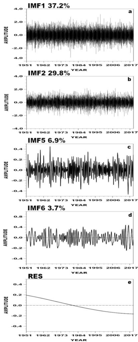
Fig.2: The intrinsic mode functions and explained variance of the daily WeMO index EMD decomposition. In the last box, the residual curve (trend).
