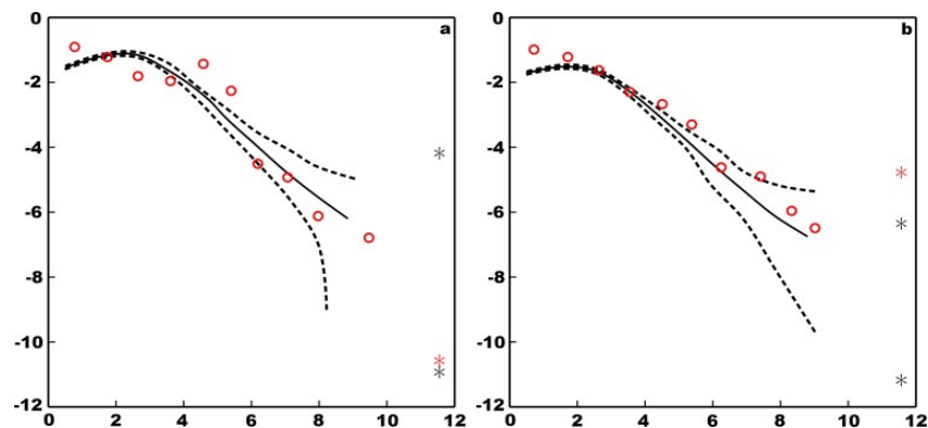
Fig. 1: a) The results of the statistical tests on the significance of the Intrinsic Mode Function of the daily MO index. The values of the variance corresponding to each IMF obtained from the Empirical Mode Decomposition of the index is depicted with red empty circles. The solid black line is the mean variance of the AR(1) ensemble and the dashed line represent the 2.5 % and 97.5 % percentiles. The axes have a natural logarithmic scale. The variance of the residual of the index is depicted with a red asterisk, while the black asterisk represents the AR(1) residuals percentile. b) As in a) but for the results of the Empirical Mode Decomposition analysis of the daily WeMO index.
