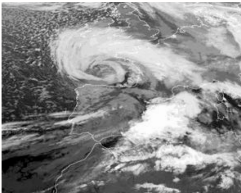
Figure 5. Infrared image, IR, from the Meteosat satellite on 24 January 2009 at 00 UTC, showing Klaus in the North of the Iberian Peninsula. Source: EUMETSAT.
