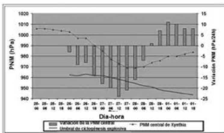
Figure 2. Xynthia's central mean sea level pressure between 25 th February at 00:00 UTC and 1 st March at 18 UTC (red triangles in hPa) and respective 24 hours variation between 26 th February at 00:00 UTC and 1 st March at 18:00 UTC (blue bars in hPa/24h) according to ECMWF analysis. The explosive cyclogenesis threshold (in magenta) according to Sanders and Gyakum (1980) is plotted for comparison during the deepening phase. Source and credit: www.eumetrain.org
