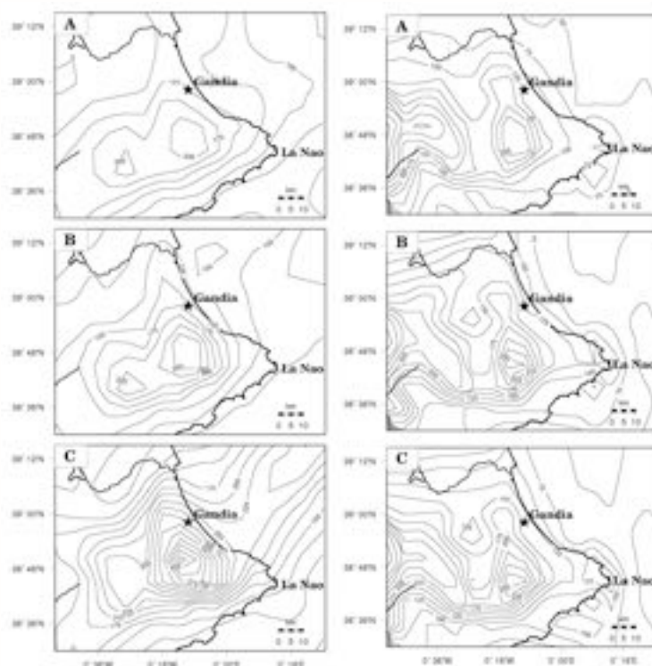
Figure 3. Total precipitation calculated by RAMS for the September 1989 event (left) and September-October 1986 event (right): (a) control, (b) ISLSCP- International Satellite Land Surface Climatology Project (monthly climatic averages of SST), and (c) satellite simulations (NOAA).
