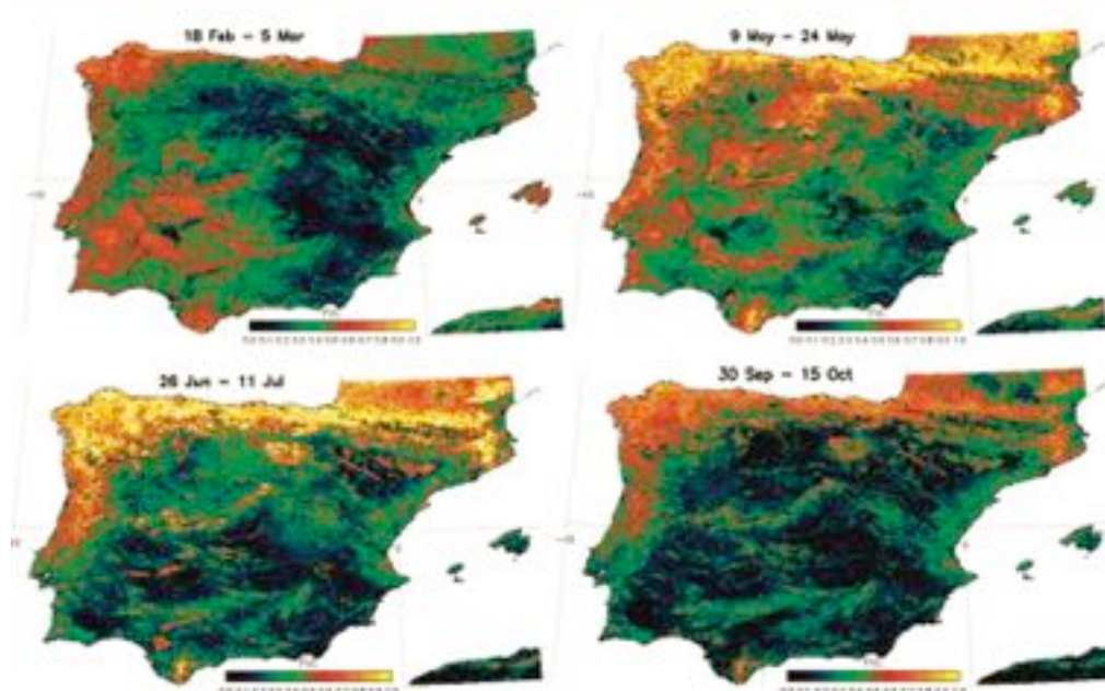
Figure 1. Monthly average (2000–2010) fractional vegetation cover (FVC) for the Iberian Peninsula at four different time periods.
