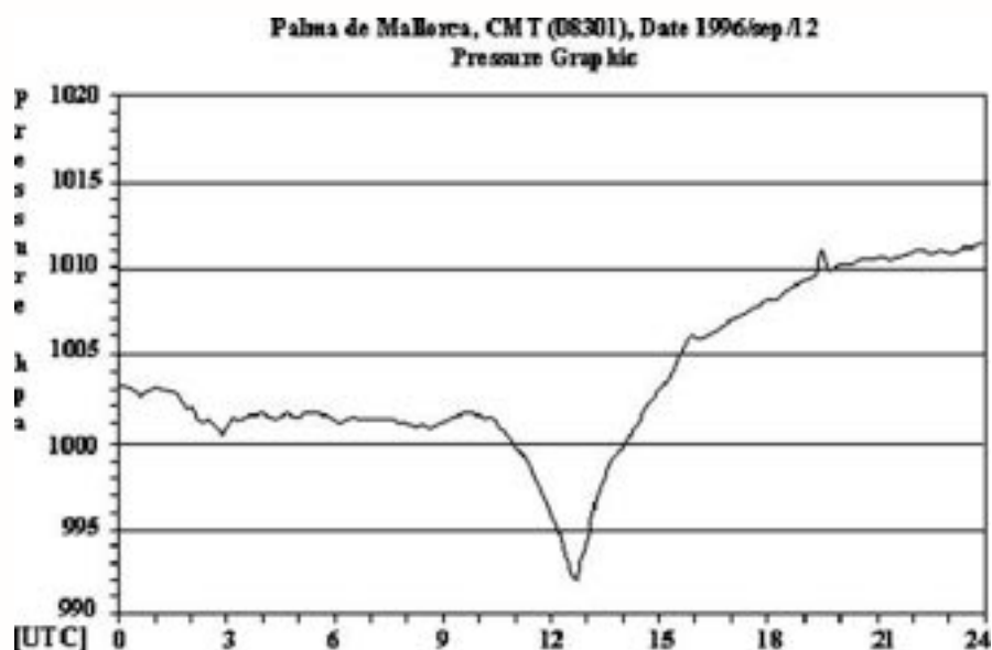
Figure 2. Barogram at Palma de Mallorca on 16 September 1996 (source AEMET).
