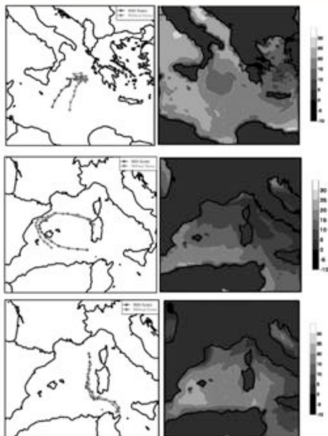
Figure 6. Simulated trajectories and spatial distribution of sensible and latent heat fluxes ( 10^3 J/kg according to the scale of grey shadings) of an event of the first group (upper row), second group (central row) and third group (lower row) (from Tous et al. , 2013).
